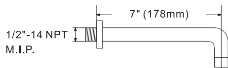
Bath spout / Bec de bain SH-157
